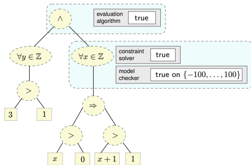
Fig. 2. An illustration of an abstract syntax tree corresponding to the logical formula “ (\forall y \in \mathbb{Z}, 3 > 1) \wedge (\forall x \in \mathbb{Z}, (x > 0 \Rightarrow x + 1 > 1)) ” with multiple values (produced by different components) for some subexpressions.
